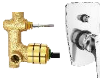
Push type single lever concealed diverter 40 mm Exposed Part with tipton & sleeve Concealed Part without sleeve Exposed Part F1025711 Concealed Part F4010201
