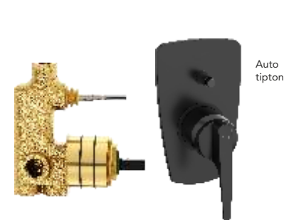
5 - Way (3 inlets + 2 outlets) Push type single lever concealed diverter Exposed Part with tipton & sleeve Concealed Part without sleeve Exposed Part F1025722SB Concealed Part F4020202
