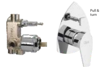
5 - Way (3 inlets + 2 outlets) single lever concealed diverter Exposed Part without tipton & sleeve Concealed Part with sleeve Exposed Part F1013711 Concealed Part F4020101
