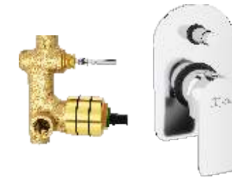
Push type single lever concealed diverter 40 mm Exposed Part with tipton & sleeve Concealed Part without sleeve Exposed Part F1016703 Concealed Part F4010201
