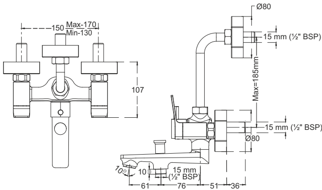
F1021403 Wall mixer (3-in-1) with arrangement for both telephonic hand shower and overhead shower with bend pipe
