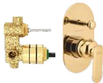
High flow single lever concealed diverter Exposed Part with tipton & sleeve Concealed Part without sleeve Exposed Part F1018901FG Concealed Part F4030501
