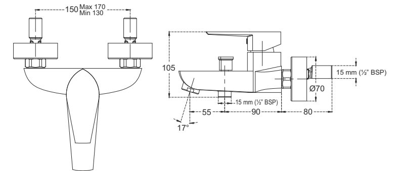
F1013414 Single lever wall mixer (2-in-1) with provision for telephonic shower arrangement
