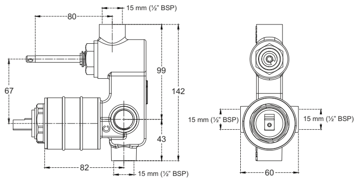
F4030501 Concealed body for high flow single lever concealed diverter system consisting of 45 mm cartridge with button Assembly,
