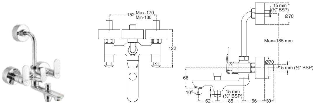
F1018403 Wall mixer (3-in-1) with arrangement for both telephonic hand shower and overhead shower with bend pipe
