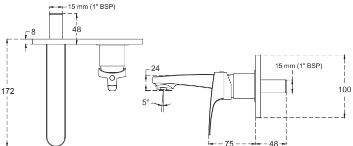
Wall mounted single lever basin mixer Exposed part F1025701 Concealed part F4065301
