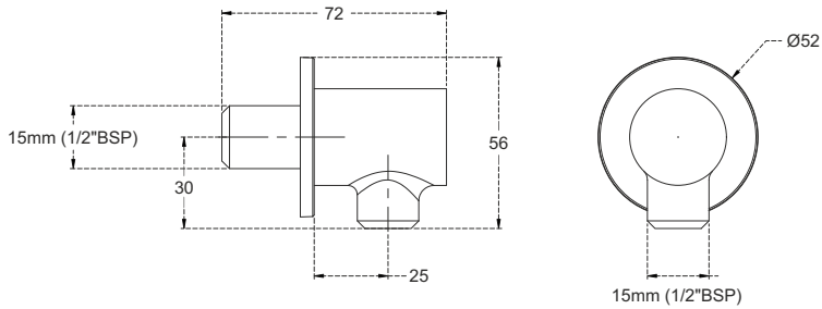
F8045103CH Wall outlet round
