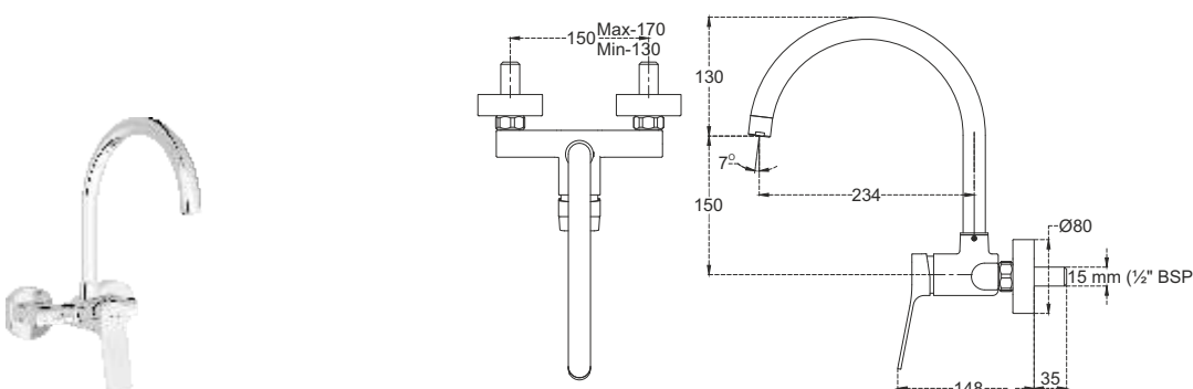
F1021502 Single lever sink mixer (wall mounted) with 235 mm (9") long swivel spout and 450 mm long braided connection pipe
