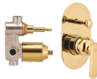
High flow single lever concealed diverter Exposed Part without tipton & sleeve Concealed Part with sleeve Exposed Part #F1018721FG Concealed Part #F4030101FG
