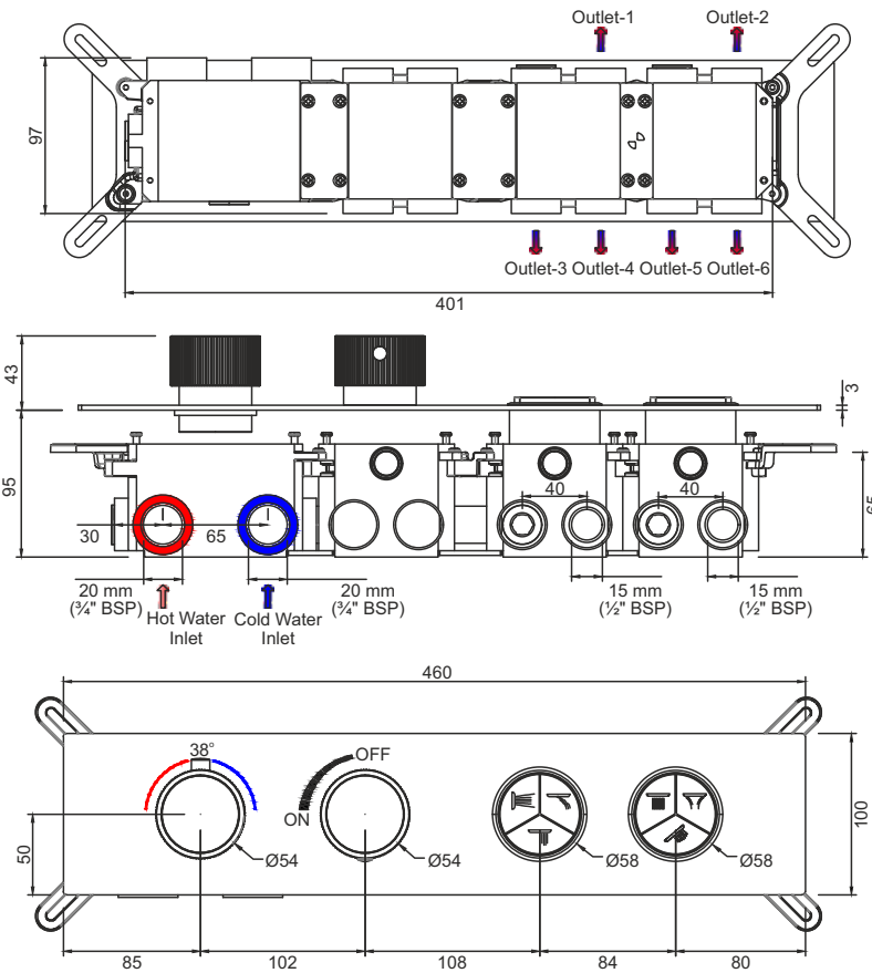
Solace Pro - 6 Outlet Thermostatic Diverter with Click type Exposed Part F8015747CH Concealed Part F4080306
