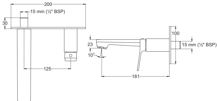
Wall mounted basin spout and operating lever Exposed part F1021653 Concealed part F4055201
