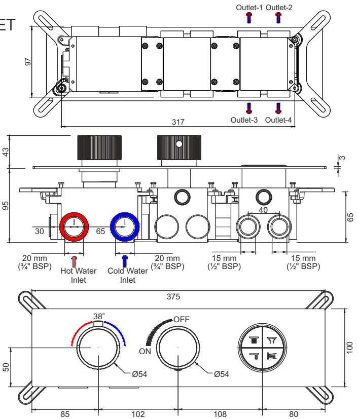
Solace Pro - 4 Outlet Thermostatic Diverter with Click type Exposed Part F8015746CH Concealed Part F4080305
