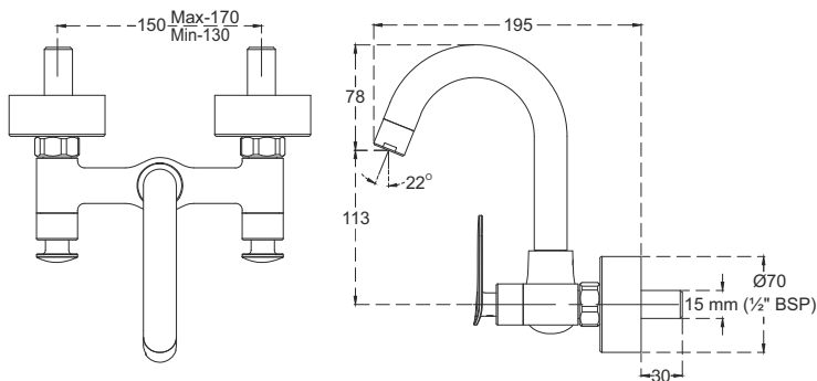
F1018501 Sink mixer (wall mounted) with 150 mm (6") long swivel spout, connecting legs and wall flanges
