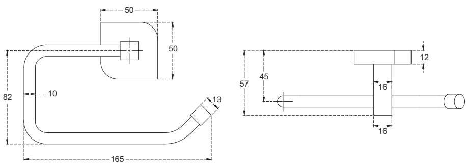
F5016104CH Towel Ring
