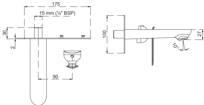
Wall mounted single lever basin mixer Exposed part F1018473 Concealed part F4065301
