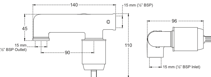
F4065301 Concealed body for wall mounted single lever basin mixer
