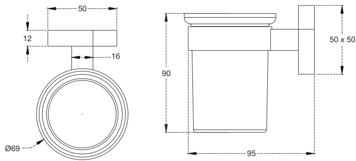
F5016106CH Tumbler Holder (Glass)
