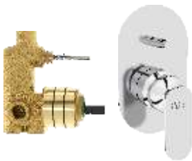
5-Way push type (3 inlets + 2 outlets) single lever concealed diverter Exposed part F1018713 ₹ 3,720 Concealed part F4020202 ₹ 4,150 Set ₹ 7,870
