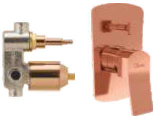
High flow single lever concealed diverter Exposed part F1021721RG ₹ 5,930 Concealed part F4030101RG ₹ 5,620 Set ₹ 11,550
