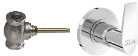
Stop cock consisting of exposed part (sleeve, lever, wall flange) and concealed part suitable for 15 and 20 mm pipeline with inner head Exposed part F1013351 ₹ 1,690 Concealed part-15 mm F4050102 ₹ 1,270 Set ₹ 2,960 Light weight concealed part-15 mm F4050103 ₹ 1,110 Exposed part F1013351 ₹ 1,690 Concealed part-20 mm F4050502 ₹ 1,310 Set ₹ 3,000 Light weight concealed part-20 mm F4050503 ₹ 1,110
