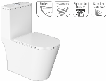
CLUER 645 x 355 x 750 mm Cat. No. S1013263 S Trap 300 mm Cat. No. S1013264 S Trap 220 mm with duroplast slim soft close seat cover
