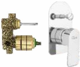
High flow single lever concealed diverter Exposed part F1016901 ₹ 3,840 Concealed part F4030501 ₹ 3,800 Set ₹ 7,640
