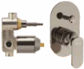
High flow single lever concealed diverter Exposed part F1018722GG ₹ 5,000 Concealed part F4030101GG ₹ 5,620 Set ₹ 10,620
