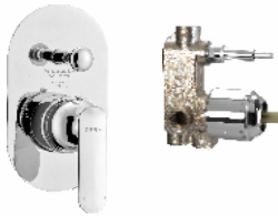
5 - Way (3 inlets + 2 outlets) single lever concealed diverter Exposed part F1018711 ₹ 2,835 Concealed Part F4020101 ₹ 4,750 Set ₹ 7,585
