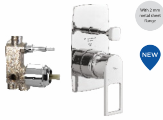
5 - Way (3 inlets + 2 outlets) single lever concealed diverter Exposed part F1099712 ₹ 3,090 Concealed Part F4020101 ₹ 4,750 Set ₹ 7,840
