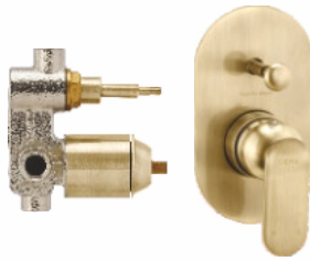
High flow single lever concealed diverter Exposed part F1018721BA ₹ 4,540 Concealed part F4030101BA ₹ 5,620 Set ₹ 10,160
