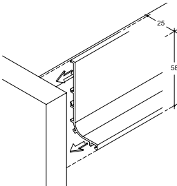
Battuta fianco terminale anta base / Horizontal groove against end of side panel / Feuillure porte module de base.
