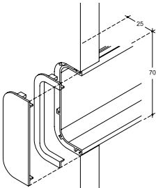
Passante fianco terminale cestoni base / Double horizontal groove at end of side panel / Traversant grands bacs de base.
