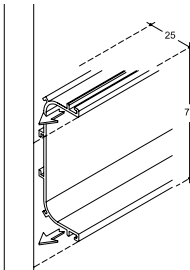
Battuta fianco terminale cestoni base / Double horizontal groove against end of side panel / Feuillure grands bacs de base.
